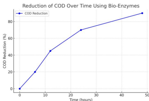
Fig. 1. Reduction of COD over time using bio-enzymes
