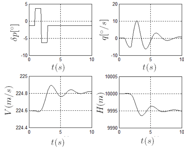
Fig. 10. Airplane Response to one doublet of elevator, V=224.6\text{m/s} , EA= 0.00\text{c}
