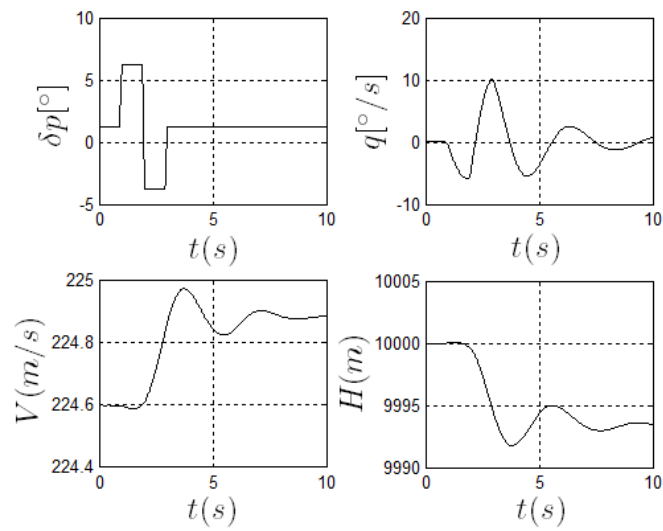
Fig. 12. Airplane Response to one doublet of elevator, V=224.6\text{m/s} , EA= -0.25c
