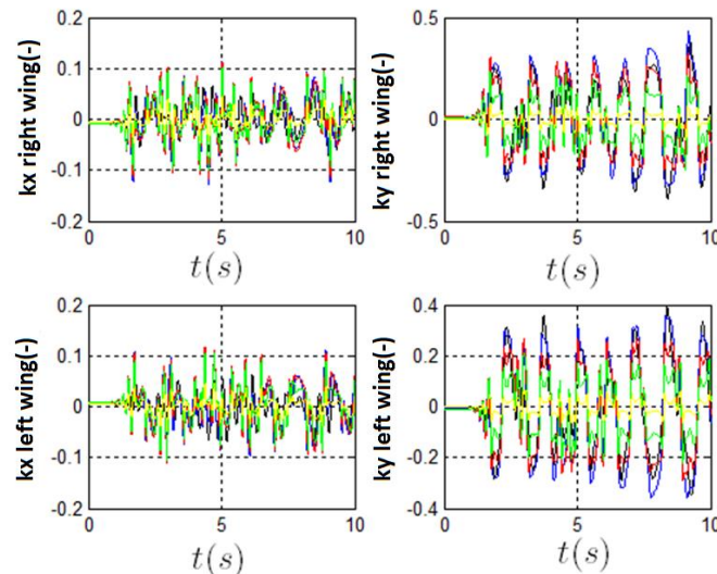
Fig. 21. Bending and Twist Wing response to one doublet of elevator, V=524.6\text{m/s} , EA= -0.25\text{ c}
