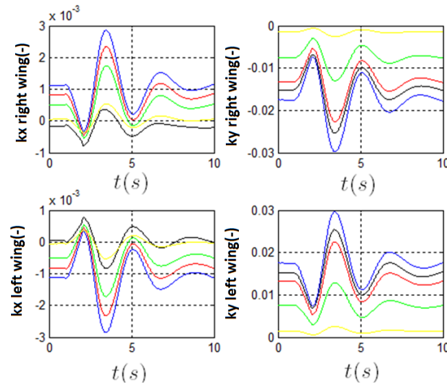
Fig. 11. Bending and Twist Wing response to one doublet of elevator, V=224.6\text{m/s} , EA= 0.0\text{ c}
