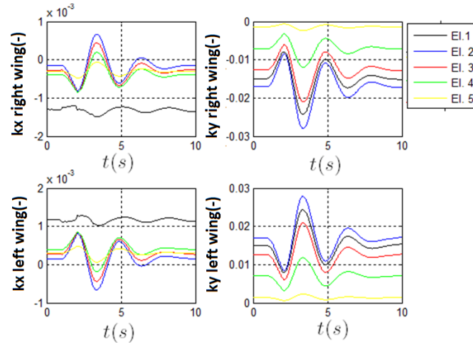
Fig. 9. Bending and Twist Wing response to one doublet of elevator, V=224.6\text{m/s} , EA=0.25\text{ \%c}
